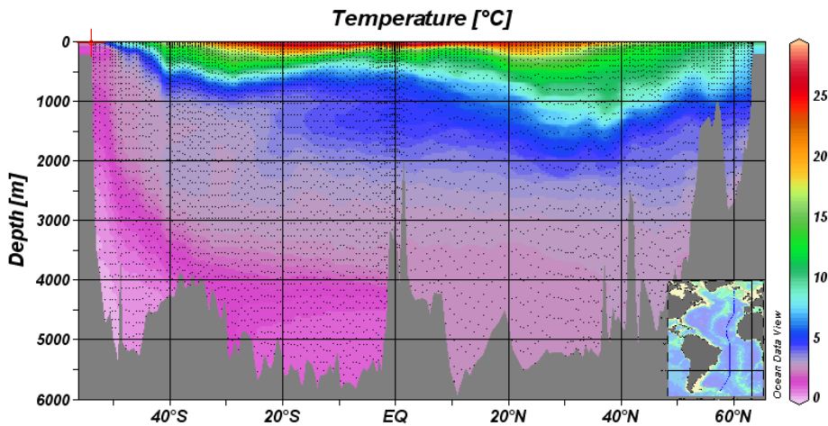
Fig. 2. North-south vertical cross section of ocean temperature with depth in the Atlantic Ocean, showing that over half of the ocean depth is colder than 40 F (about 5 C on the color scale), even in the tropics.
