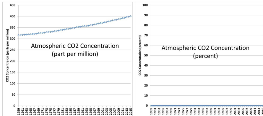
Fig. 1. The atmospheric concentration of carbon dioxide at Mauna Loa, HI between 1959 and 2015, in parts per million (left panel), and as a percent of the atmosphere (right panel).
