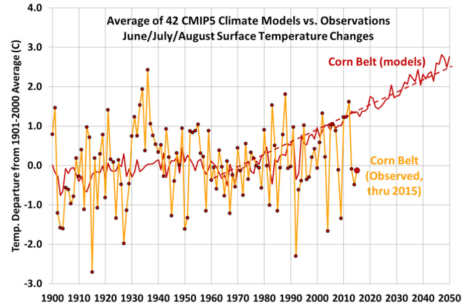
Fig. 10. Comparison of the average surface temperature predictions across 42 climate models versus observations for the primary U.S. Corn Belt states (IA, IL, IN, KS, MI, MN, MO, NE, ND, OH, SD, WI) also shows the models are warming faster than the real climate system (official NOAA data).
