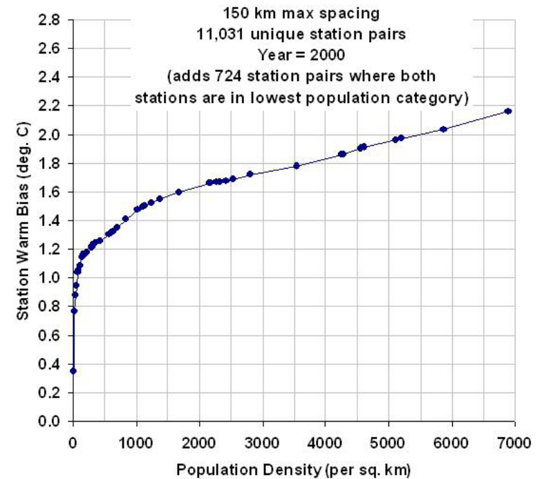
Fig. 4. Localized warming (Urban Heat Island effect) at temperature monitoring stations occurs as population density increases, as seen in this analysis of one year of daily temperature data from all reporting stations in the world. Note the most rapid warming occurs at the lowest population densities.
