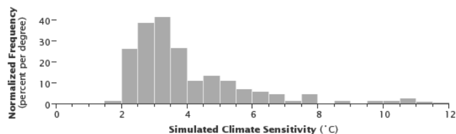
Fig. 11. Frequency histogram of the climate sensitivities of ~100 climate models tracked by the IPCC, revealing large uncertainty in how much warming we can eventually expect from a doubling of atmospheric carbon dioxide late in this century.
