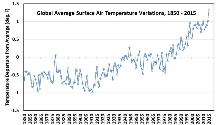
Fig. 8. Surface-based thermometer estimates of global average temperature, after adjustments, show about a 1.5 F temperature increase over the last 150 years (HadCRUT4 data).
