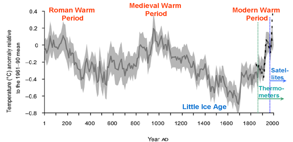
Fig. 3. Estimates of Northern Hemisphere average temperature over the last 2,000 years. Note that most centuries experienced natural episodes of warming or cooling.
