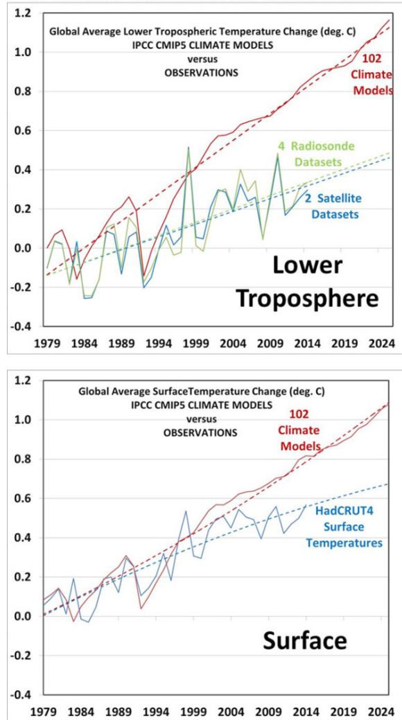
Fig. 9. Comparison between climate model “predictions” and actual observations of global average temperature since 1979 suggest that models are warming about twice as fast as the real world.
